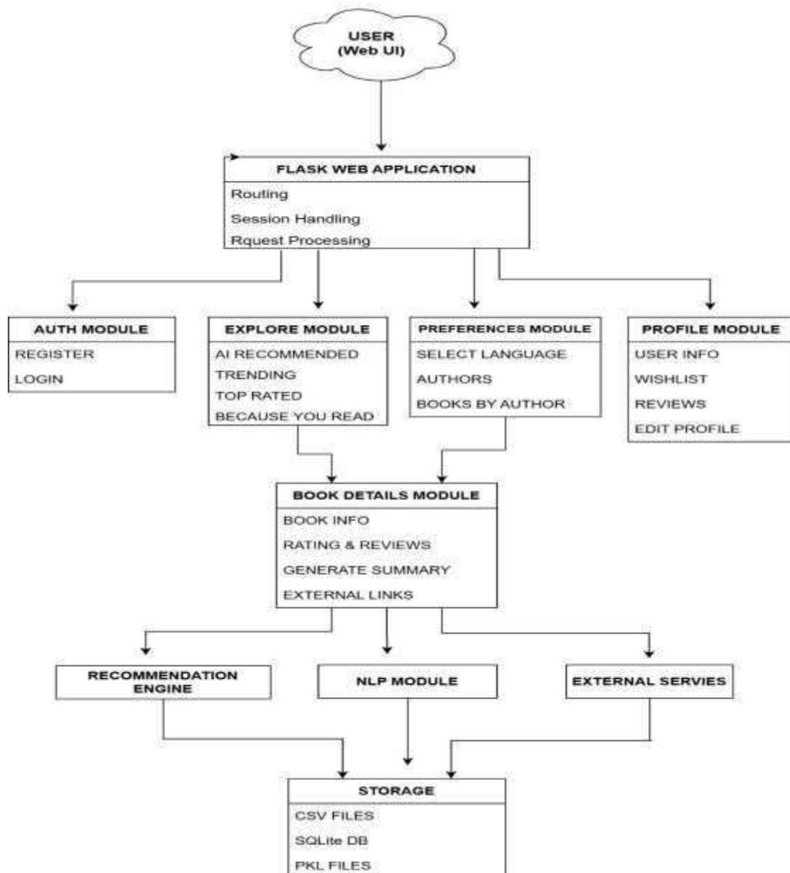
FIG 11.1 ARCHITECTURE DIAGRAM
