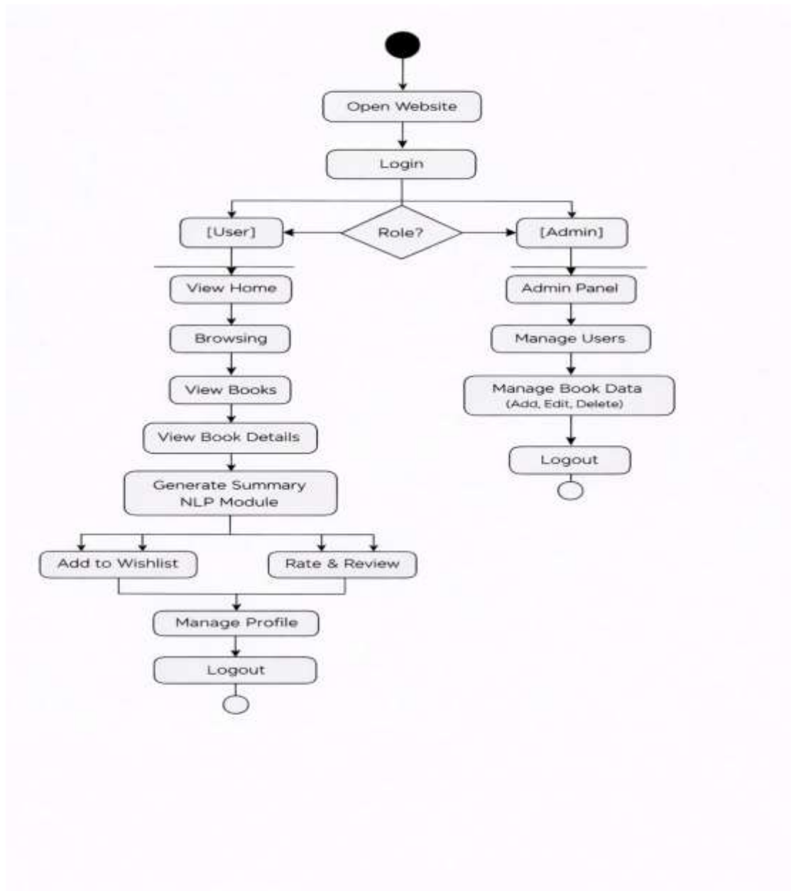
FIG 11.3.3 ACTIVITY DIAGRAM
