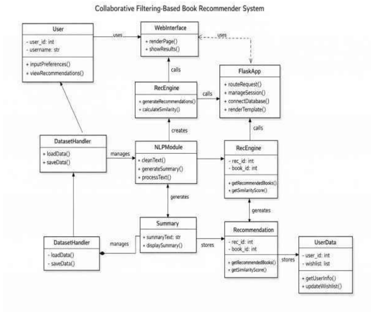
FIG 11.3.2 CLASS DIAGRAM
